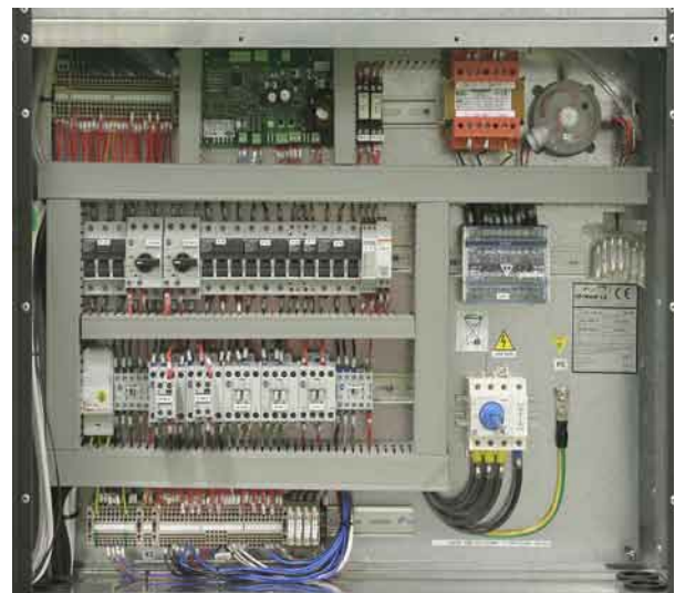
Control panel
